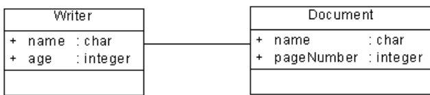
Class diagram
