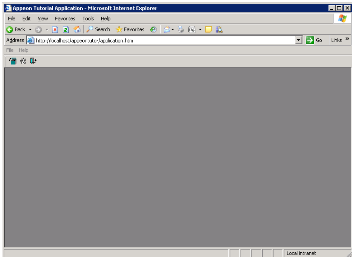
Figure 7-54: Application starts
