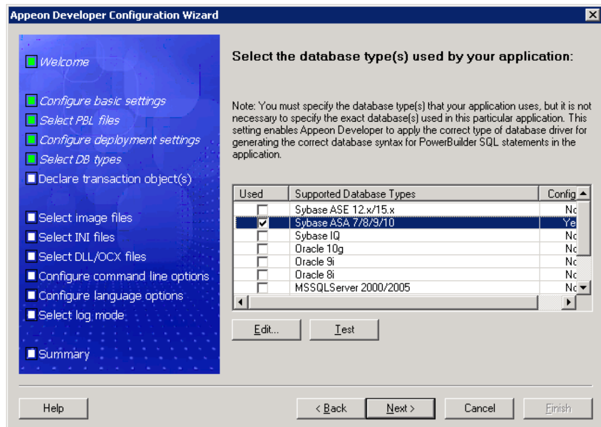
Figure 7-33: DB Type
