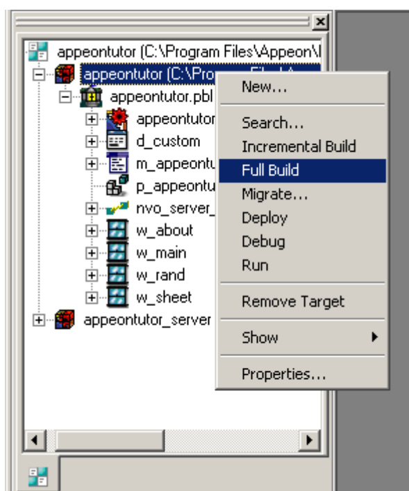
Figure 7-49: Full Build
