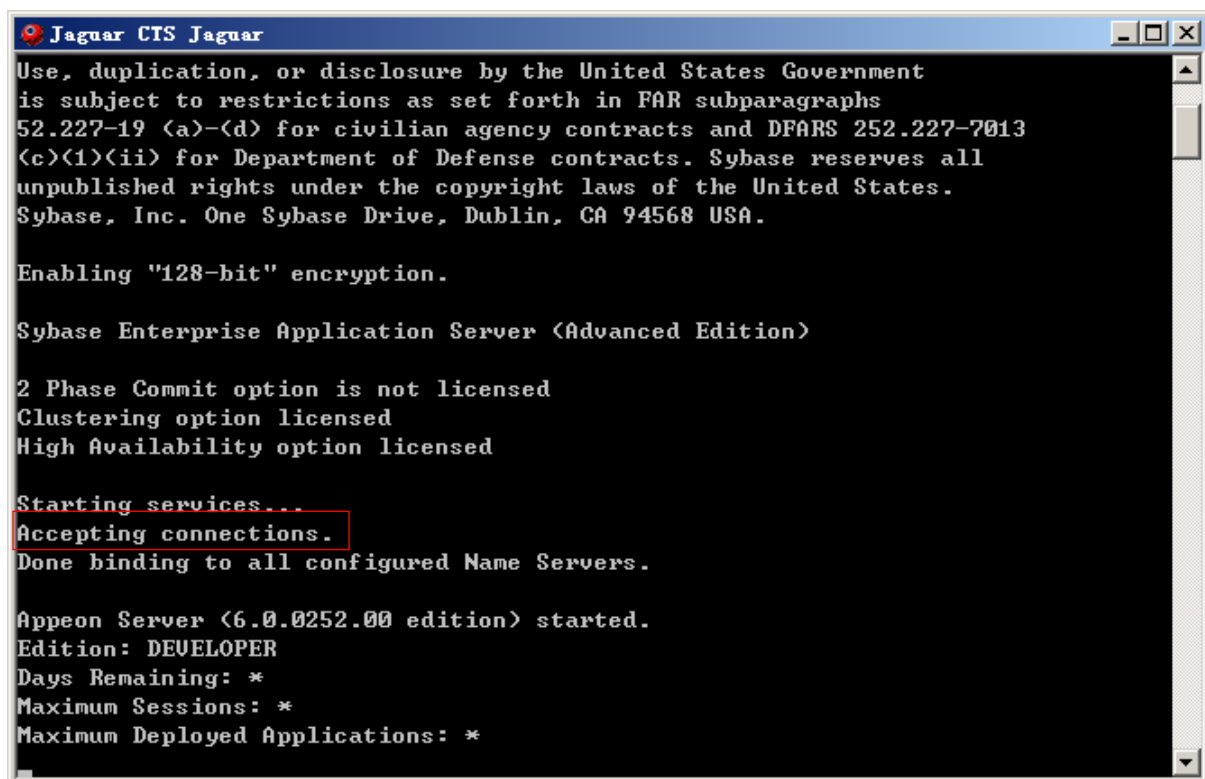
Figure 7-25: EAServer/Appeon Server
