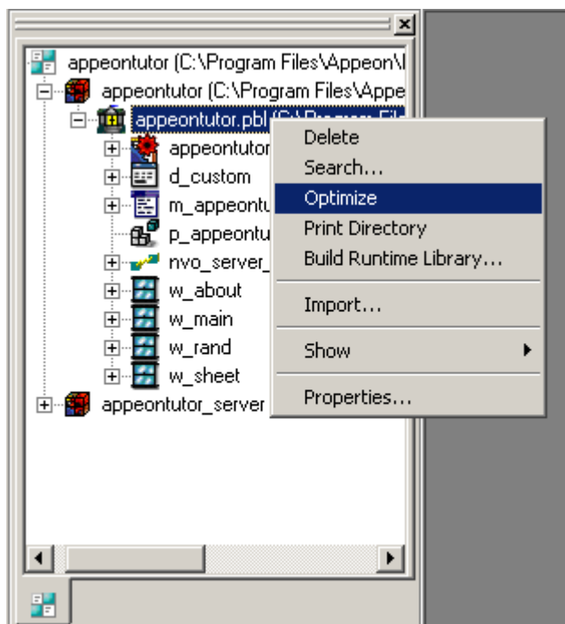
Figure 7-48: Optimize
