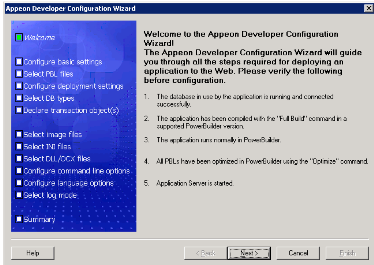
Figure 7-22: Welcome page
