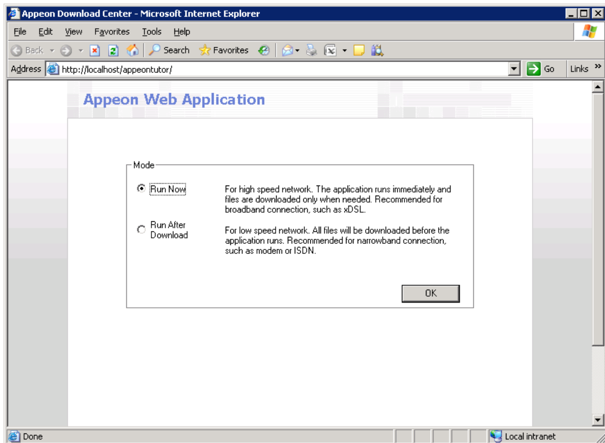
Figure 7-53: Application starts
