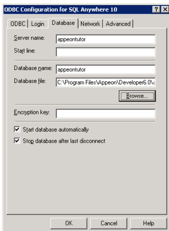
Figure 7-16: Database tab
