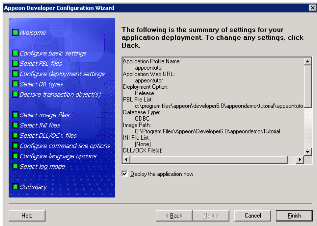
Figure 7-43: Summary
