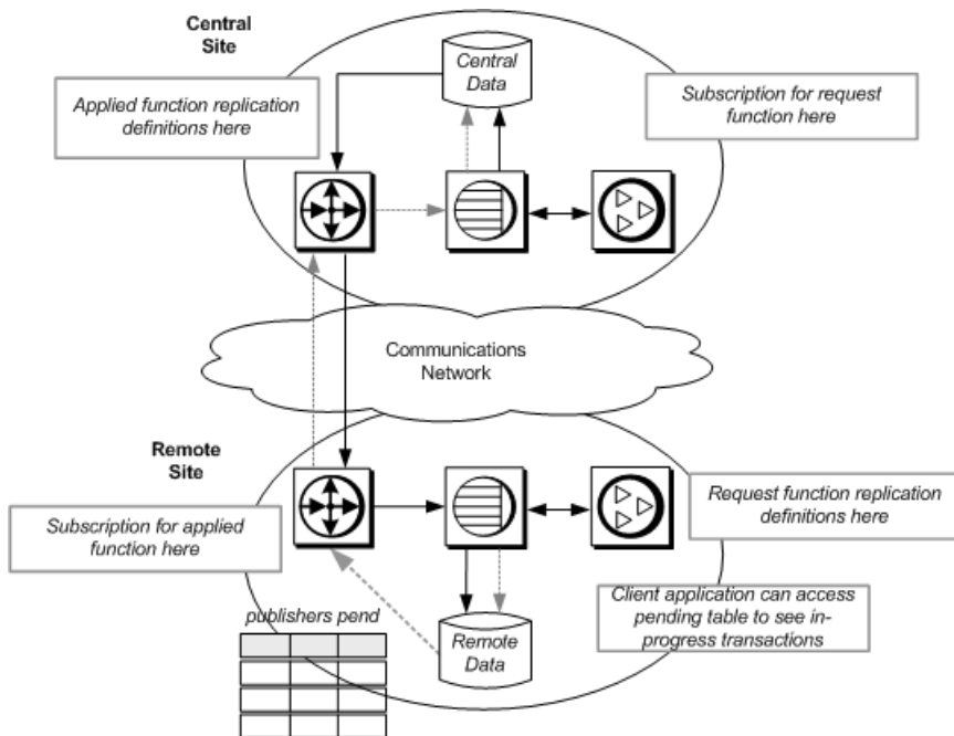
Figure 21: Request Functions and a Local Pending Table
