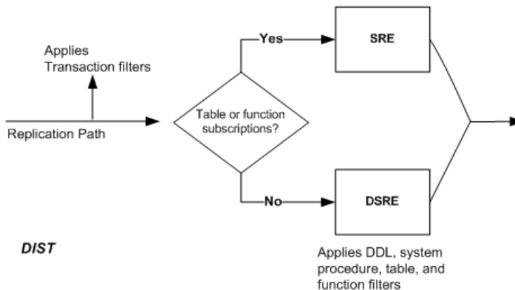
Figure 20: Evaluation of Database Replication Filters
