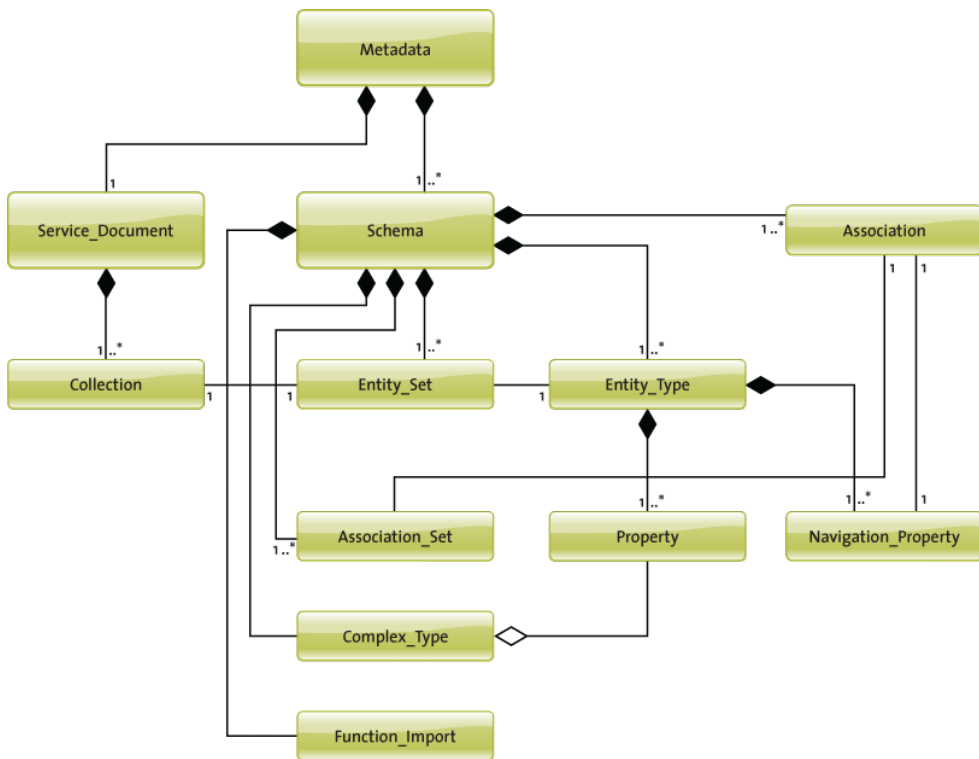
Figure 1: Object Hierarchy
