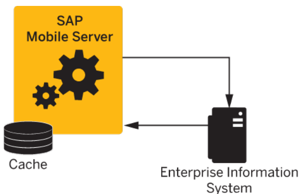
Figure 2: Load Argument
