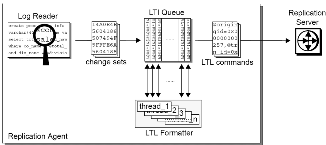
Figure 4: Replication Agent LTL Formatting
