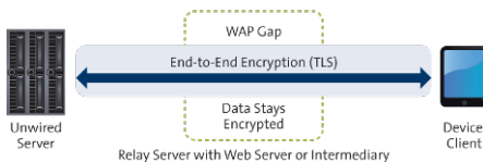
Synchronization Data Flow with End-to-End Encryption
