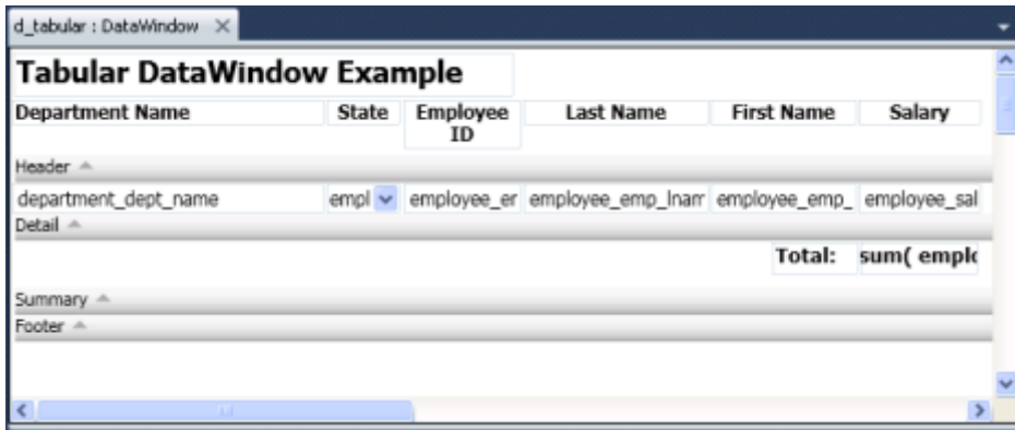
Figure 1: Design view for a tabular DataWindow object
