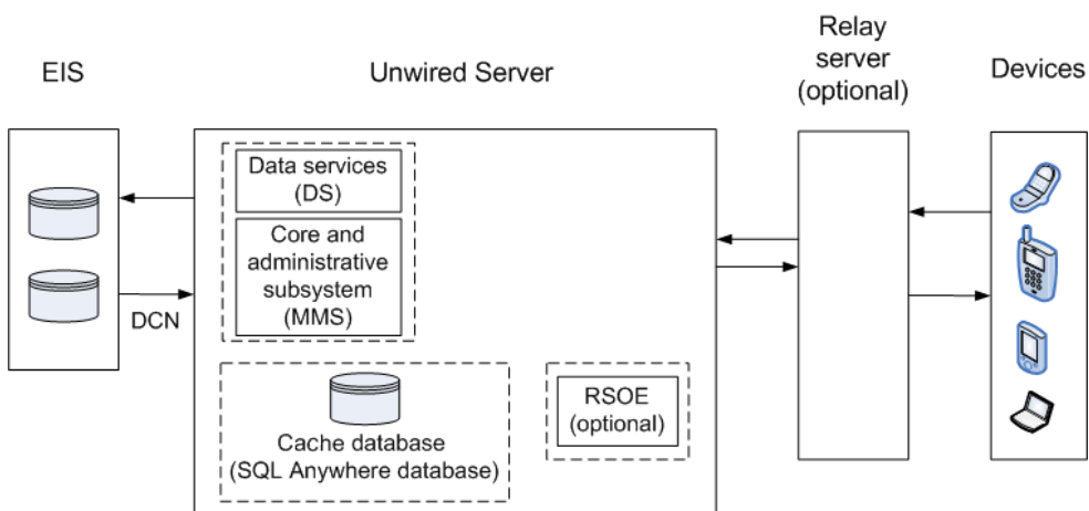
Figure 3: Replication synchronization process flow
