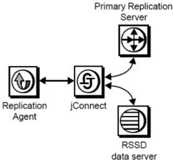
Figure 3: Replication Agent Communication with Replication Server and its RSSD
