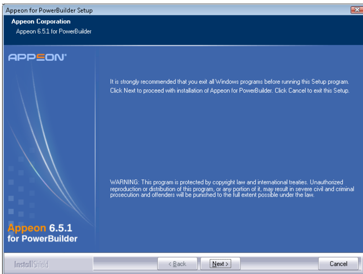
Figure 4.2: Introduction page
