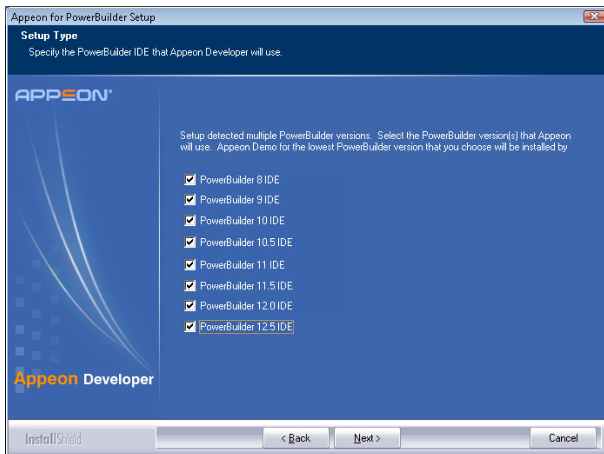
Figure 4.29: PowerBuilder IDE
