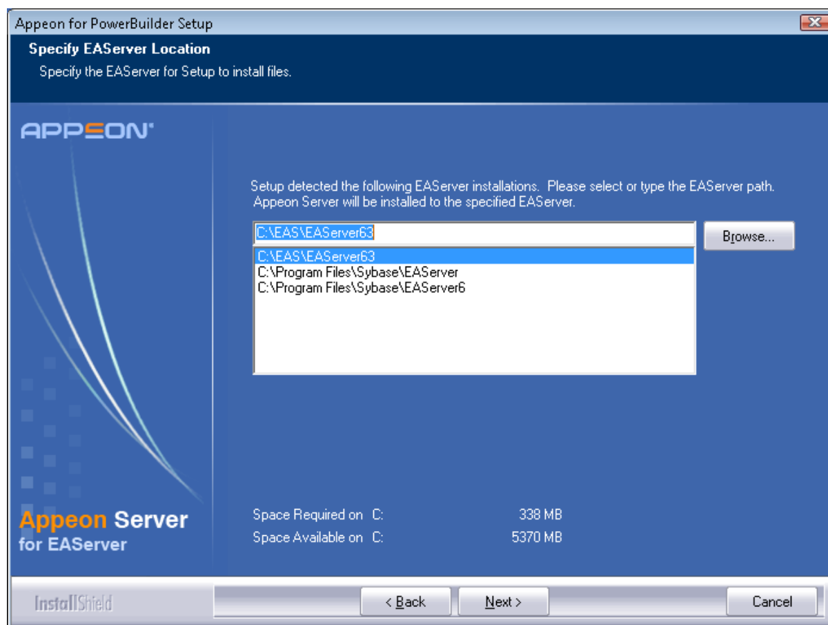
Figure 4.7: EAServer location
