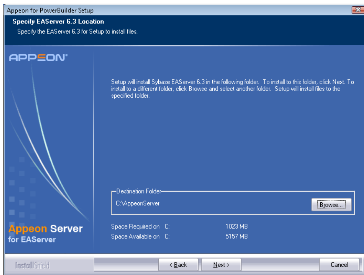
Figure 4.15: Choose location
