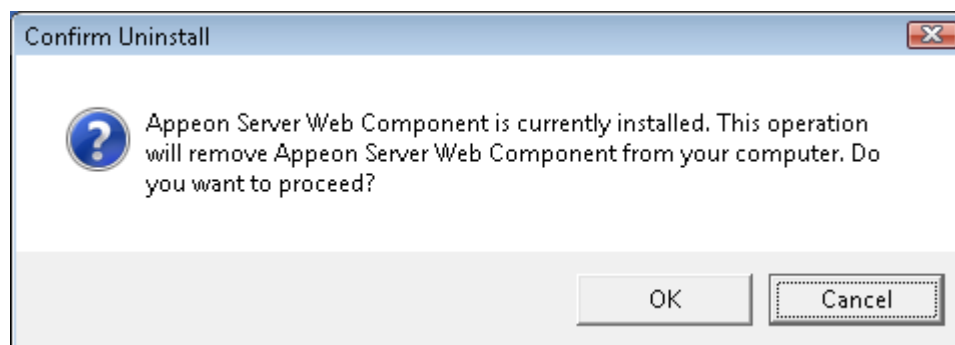
Figure 7.11: Confirm uninstall
