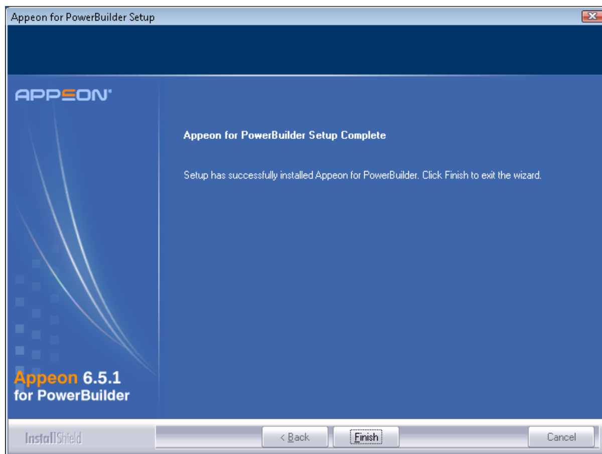
Figure 4.38: Setup Complete
