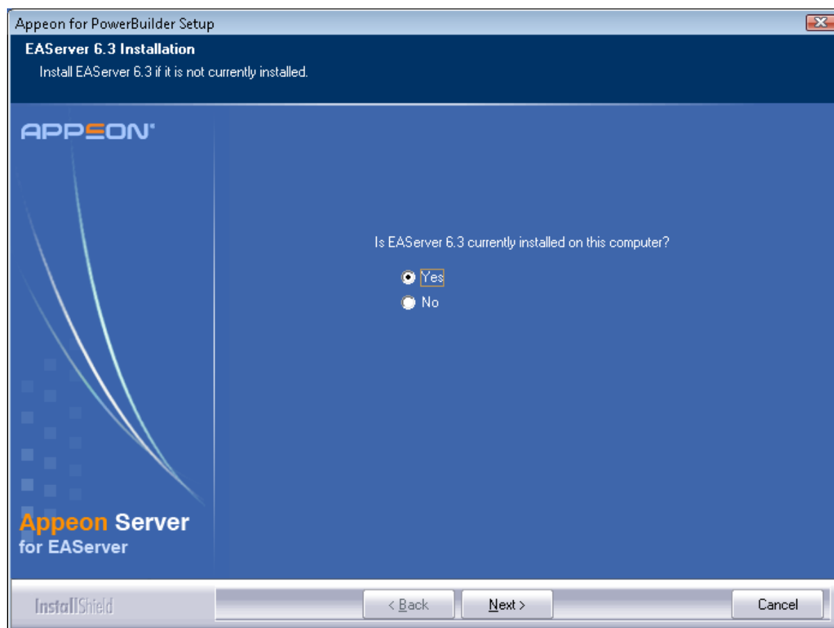
Figure 4.6: EAServer installation
