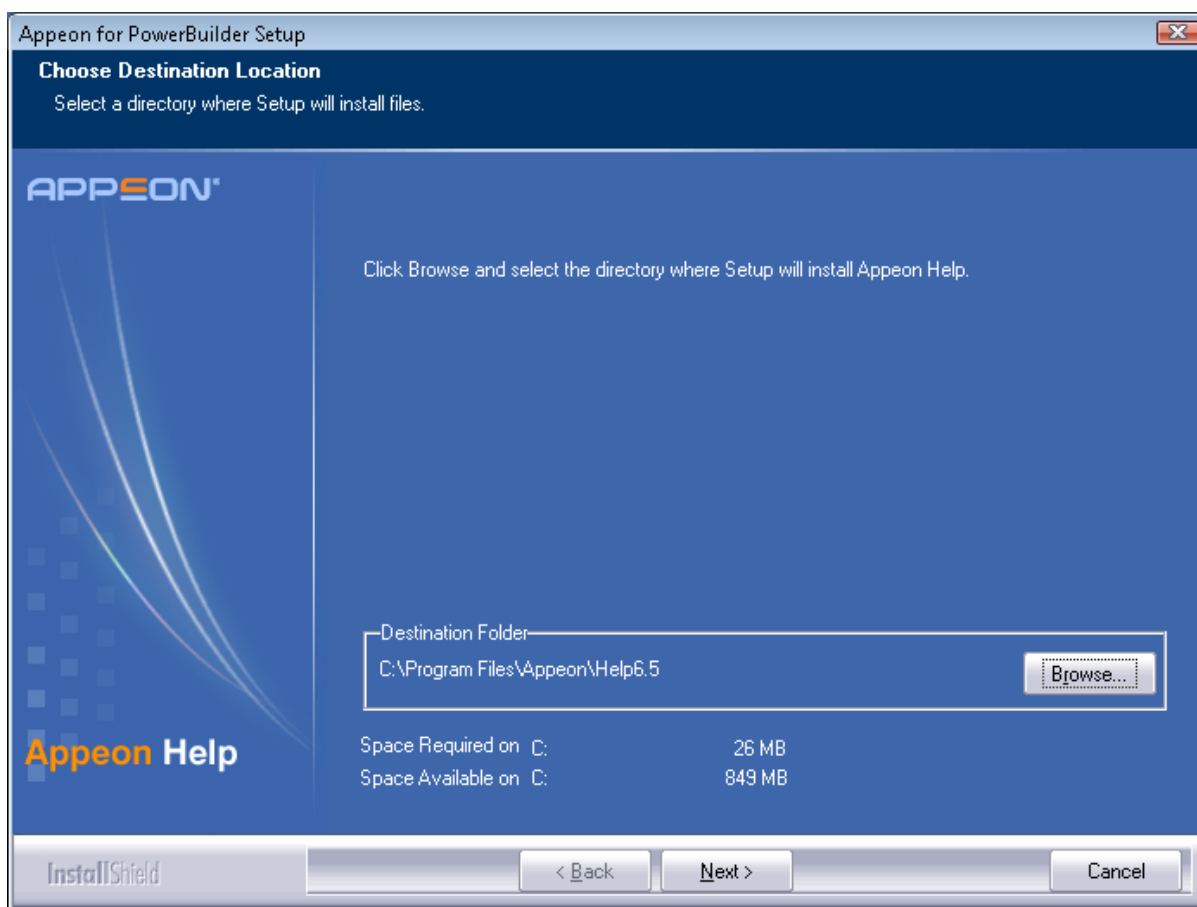
Figure 4.39: Help location
