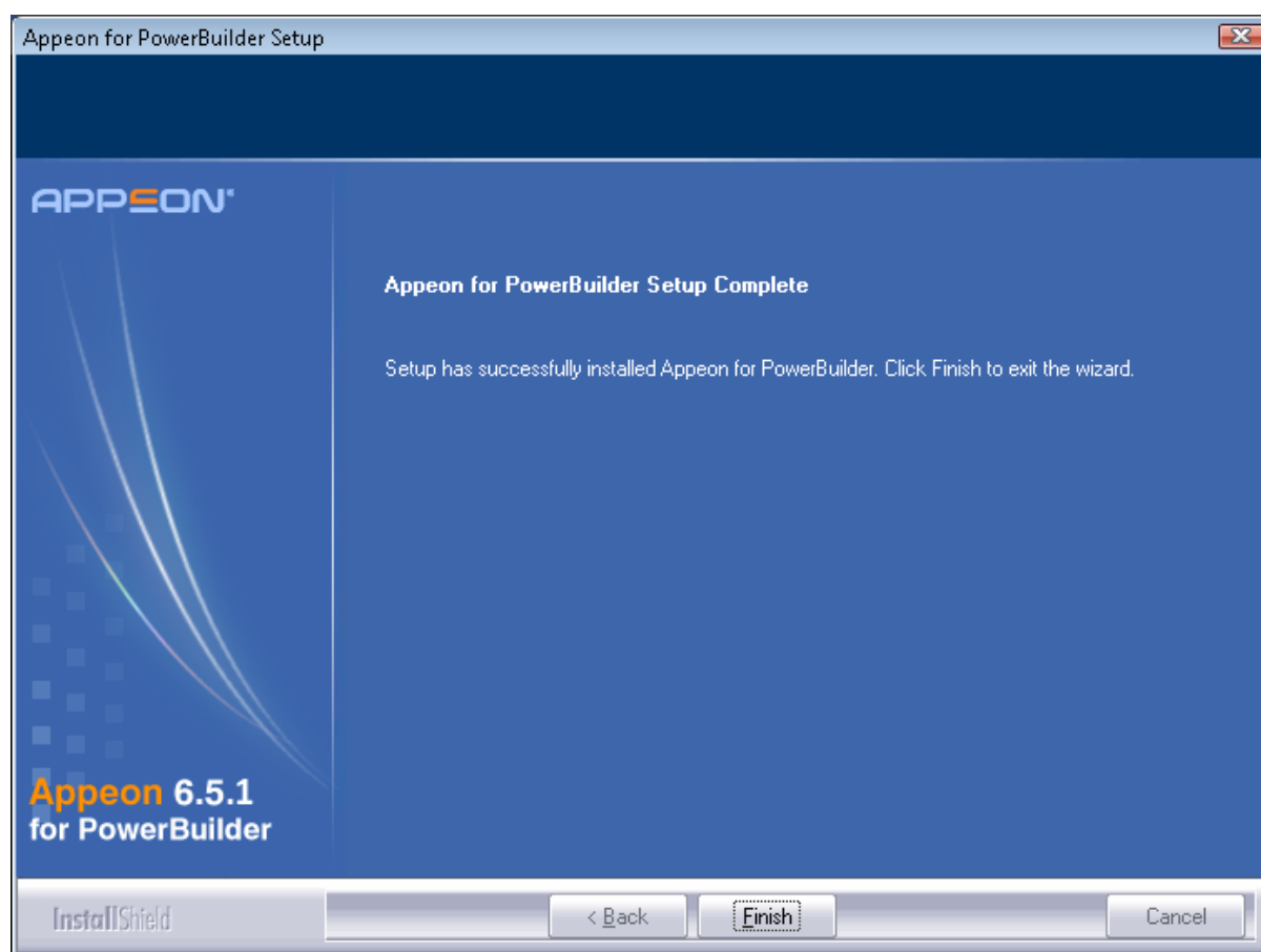
Figure 4.34: Setup Complete
