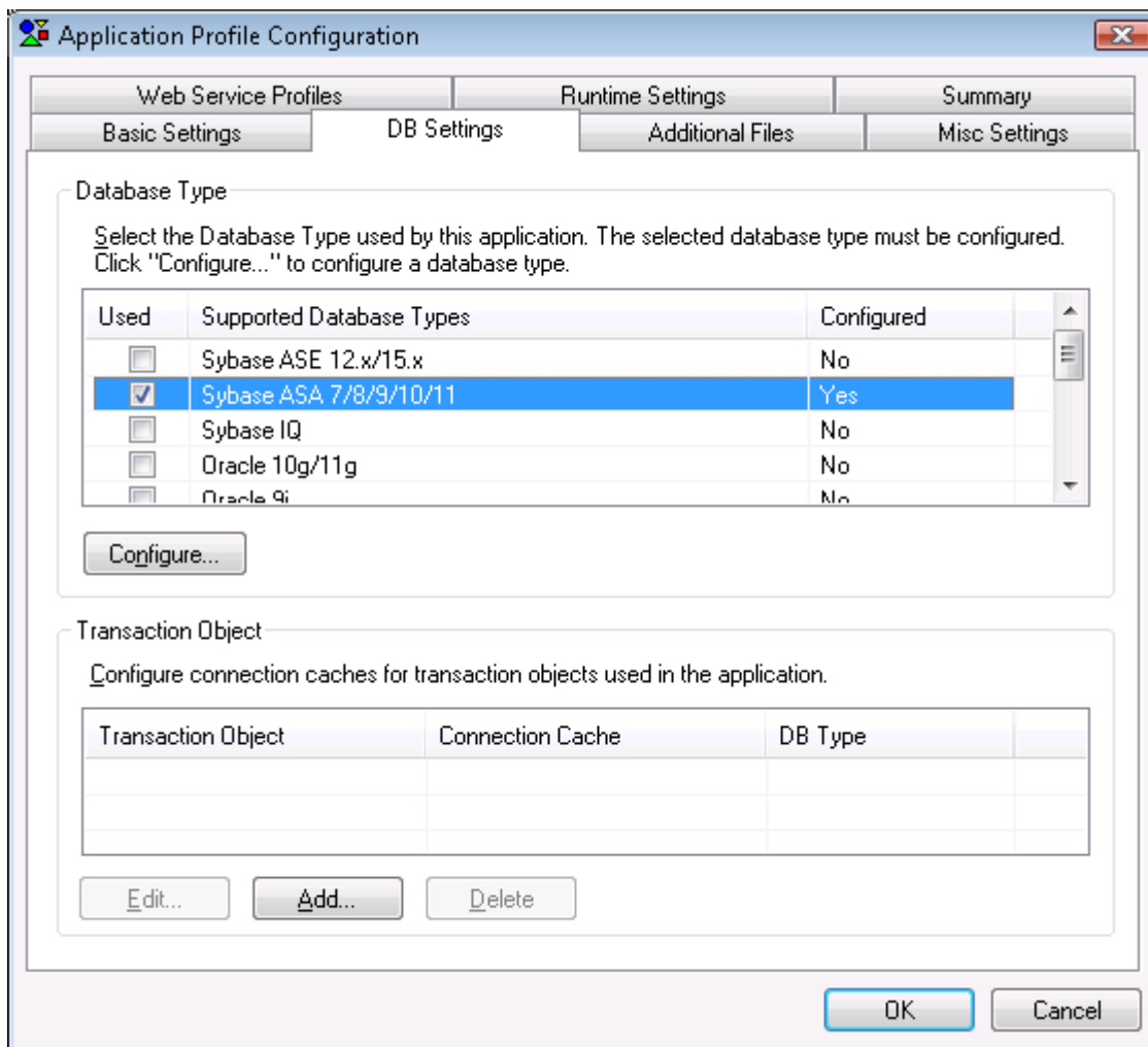
Figure 7-3: DB Type
