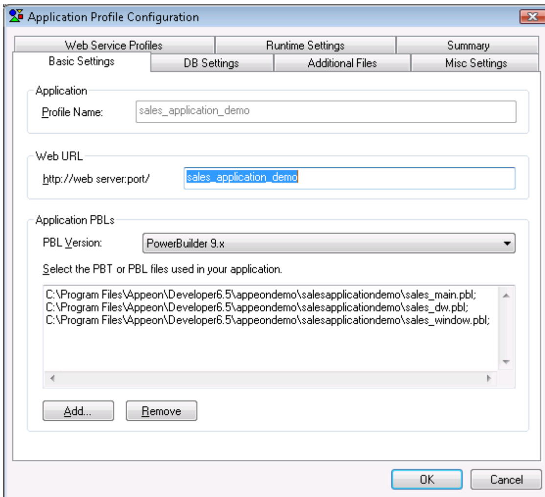
Figure 7-2: Web URL
