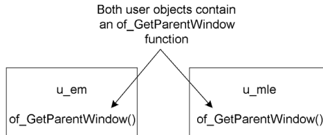
Figure 2-4: Operational polymorphism
