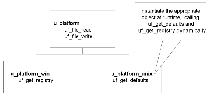
Figure 2-7: Dynamic lookup
