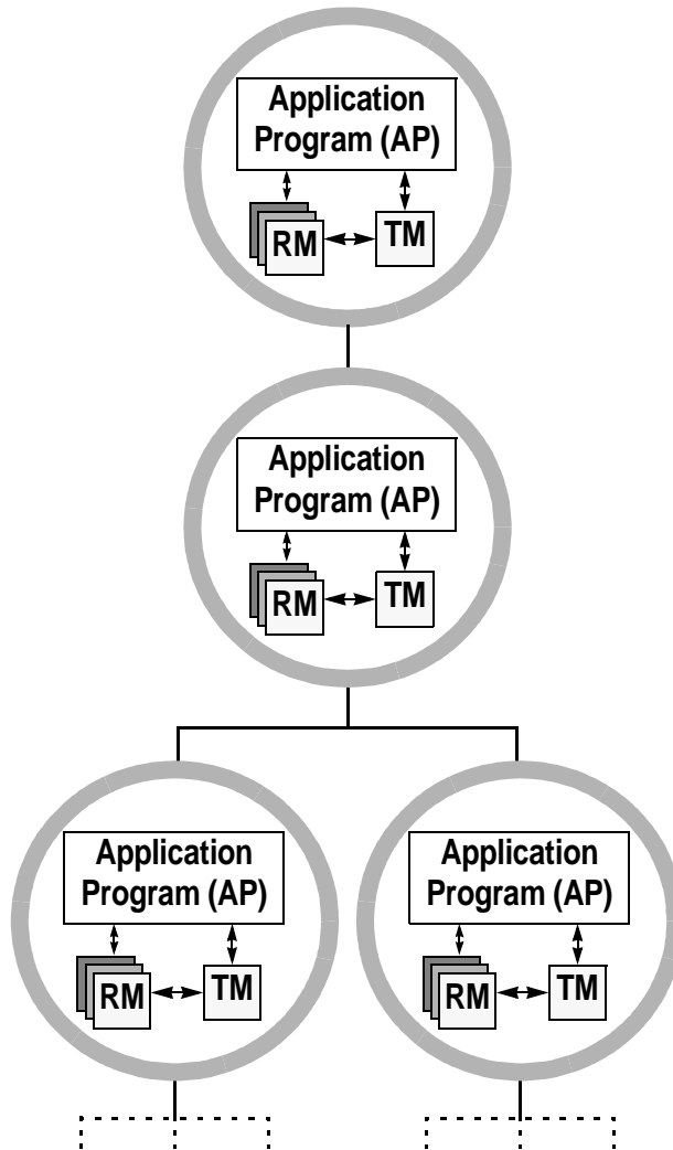
Figure 1-2: Transaction branches
