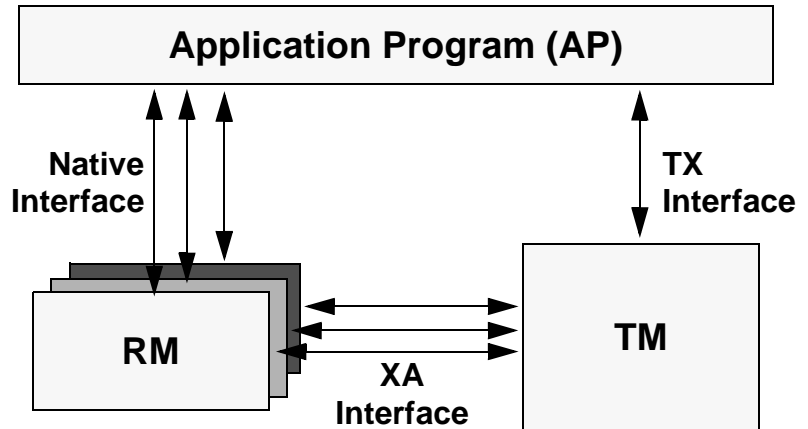
Figure 1-1: A conceptual view of the X/Open DTP model
