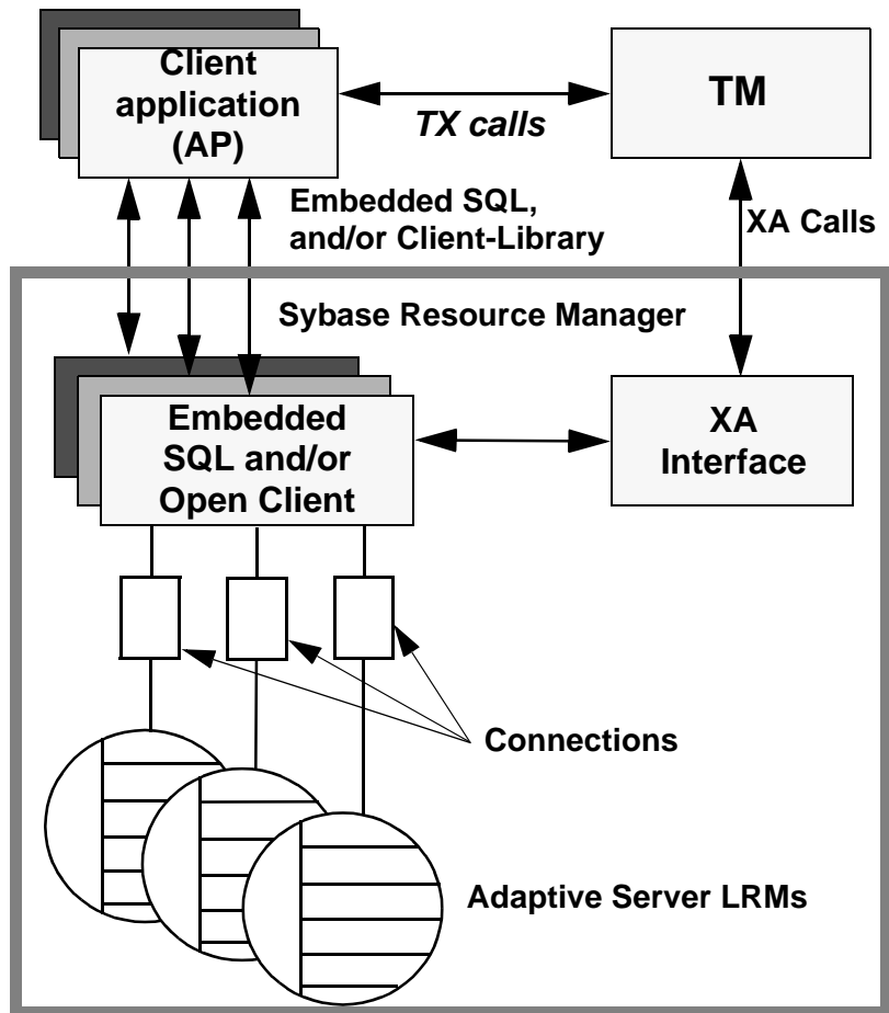
Figure 1-3: The Sybase XA DTP model
