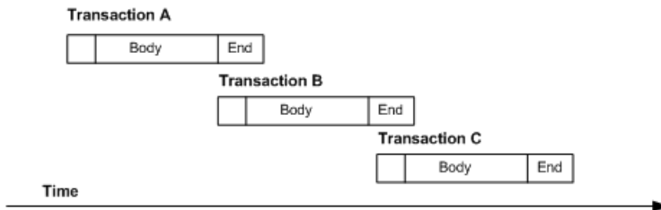
Figure 16: Thread Timing with the wait_for_commit Serialization Method
