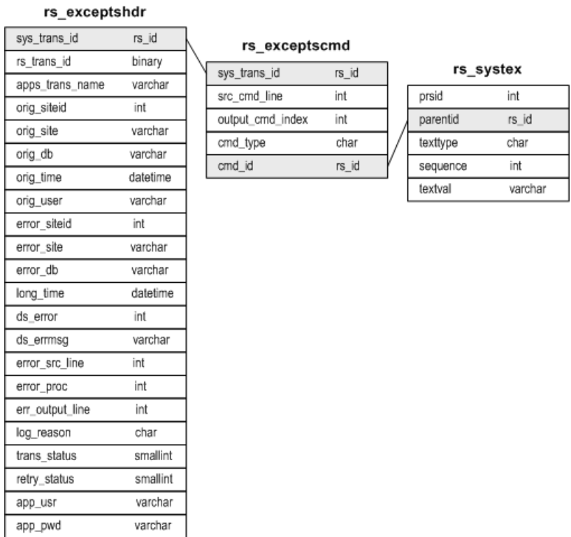
Figure 23: Exceptions Log System Tables
