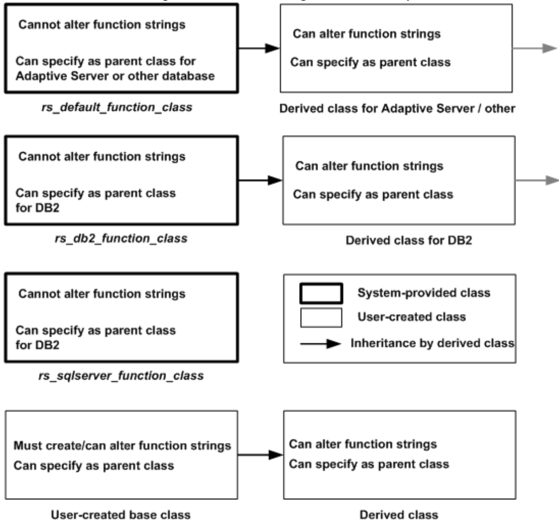
Figure 2-1: Function-string class relationships
