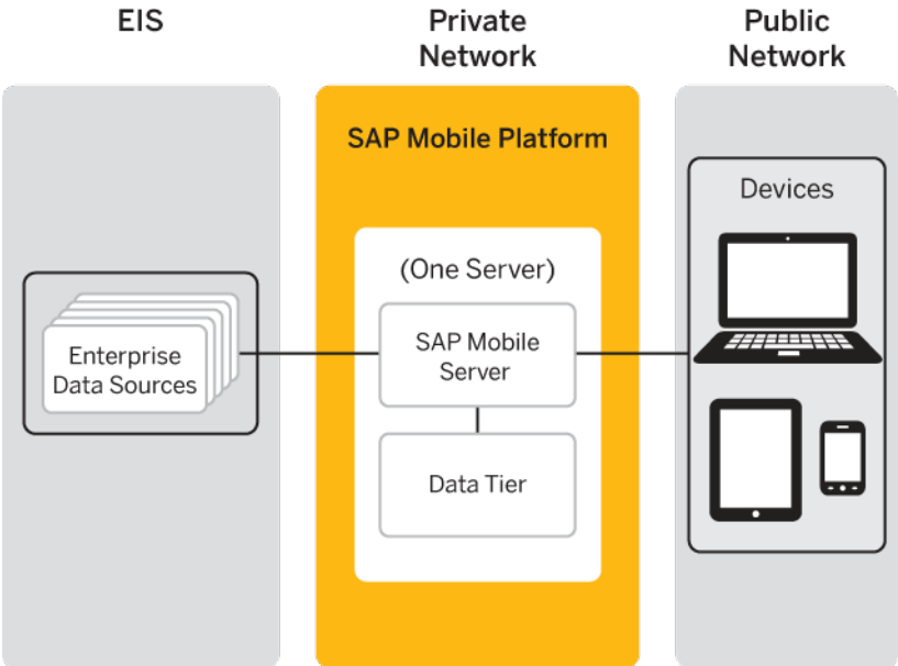
Figure 6: Single-Server Installation
