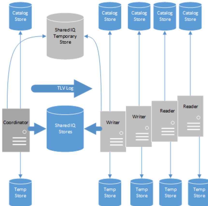
Figure 1: IQ Multiplex Architecture
