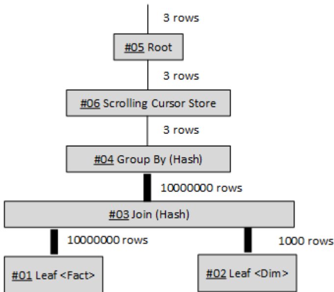
Figure 1: Sybase IQ Sample Query Plan
