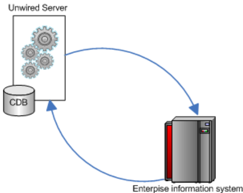
Figure 2: Load argument
