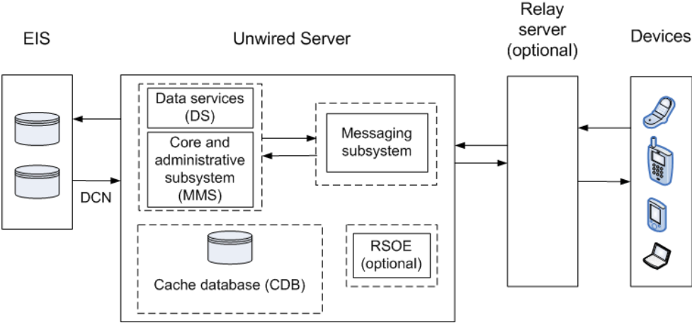
Figure 3: Message synchronization process flow
