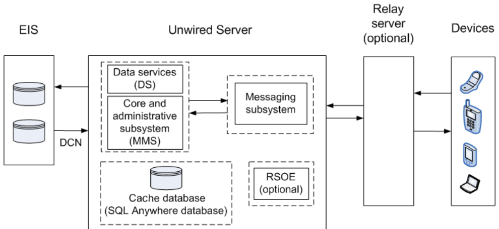
Figure 7: Cache process flow
