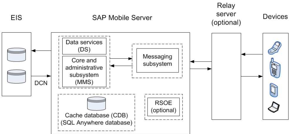
Figure 2: Sybase Unwired Platform communications
