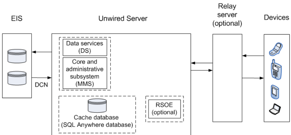
Figure 13: Replication synchronization process flow
