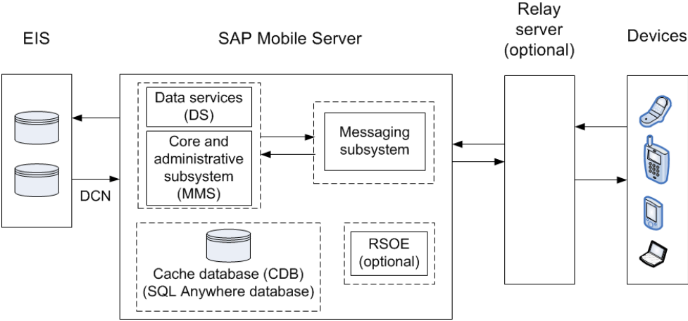
Figure 4: Message synchronization process flow
