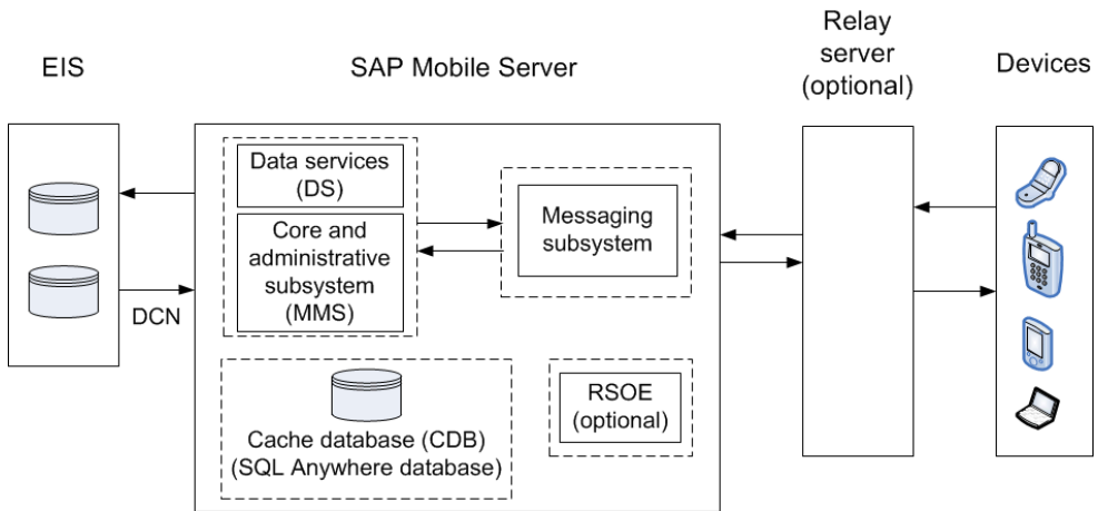
Figure 16: Message synchronization process flow
