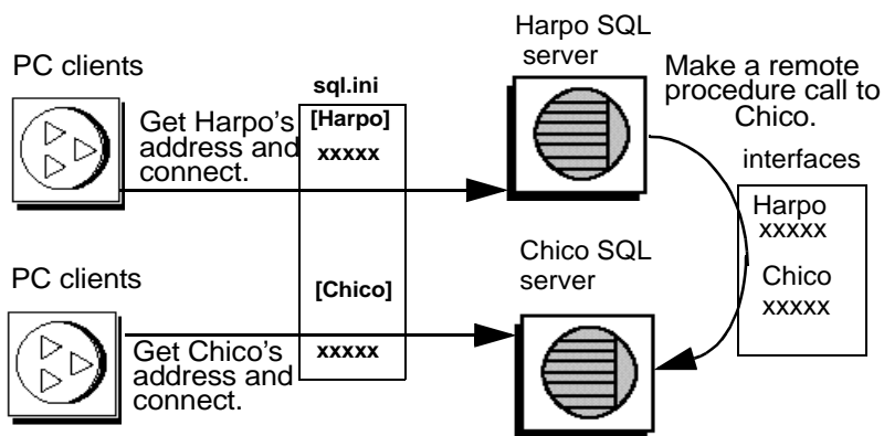
Figure 20-1: Establishing network connections in a heterogeneous environment
