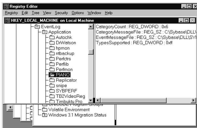
Figure 7-2: Registry key
