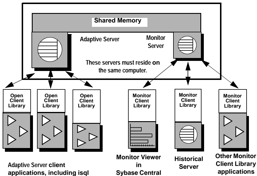
Figure 1-1: Adaptive Server Enterprise Monitor architecture
