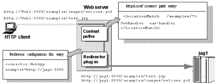
Figure 4-3: “examples” requests are redirected to EAServer
