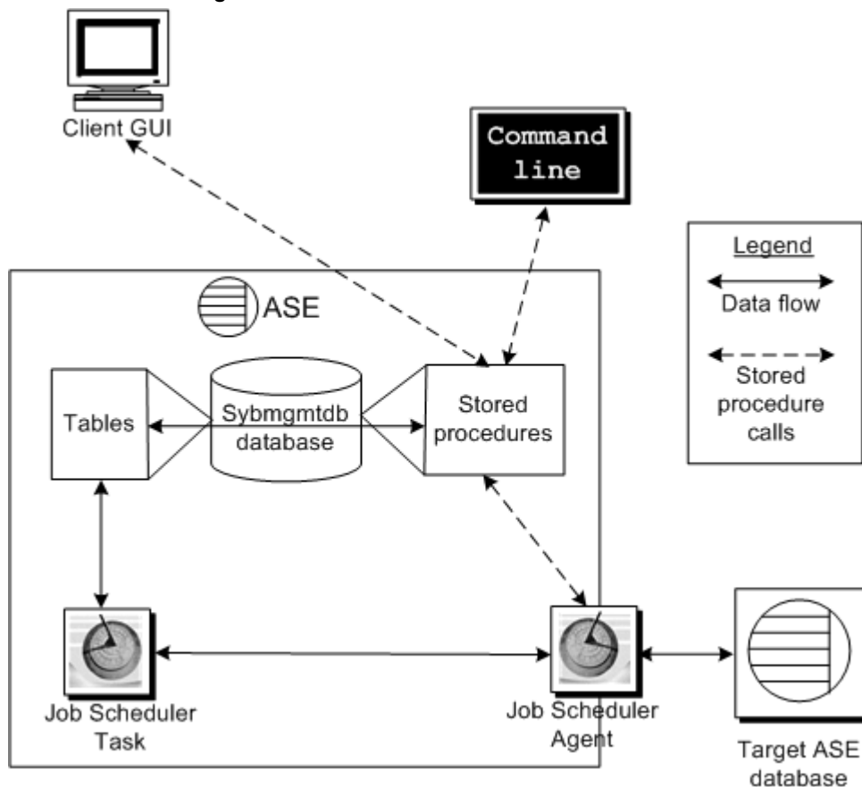
Figure 1-1: Job Scheduler architecture
