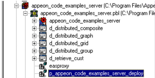
Figure 5-2: p_appeon_code_examples_server_deploy project
